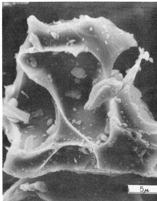
B. Vesiculated shards, X 3,200, SEM photo.
