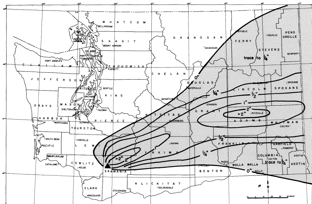
Figure 7.—Ash depths of Mount St. Helens, May 18, 1980, eruption—Washington State.
